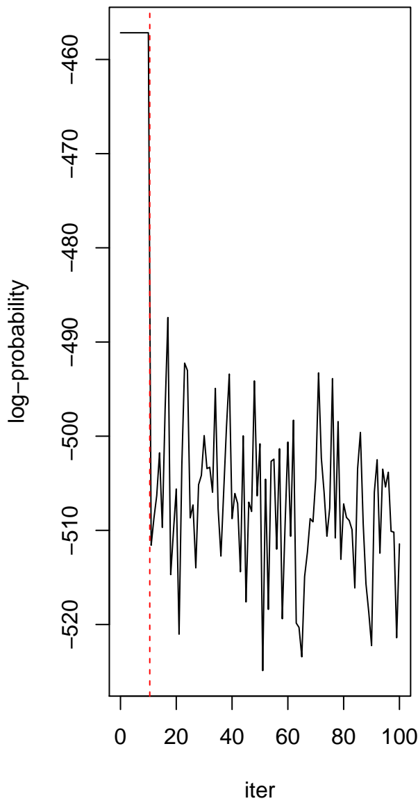
Log-Probability Trace Plot
