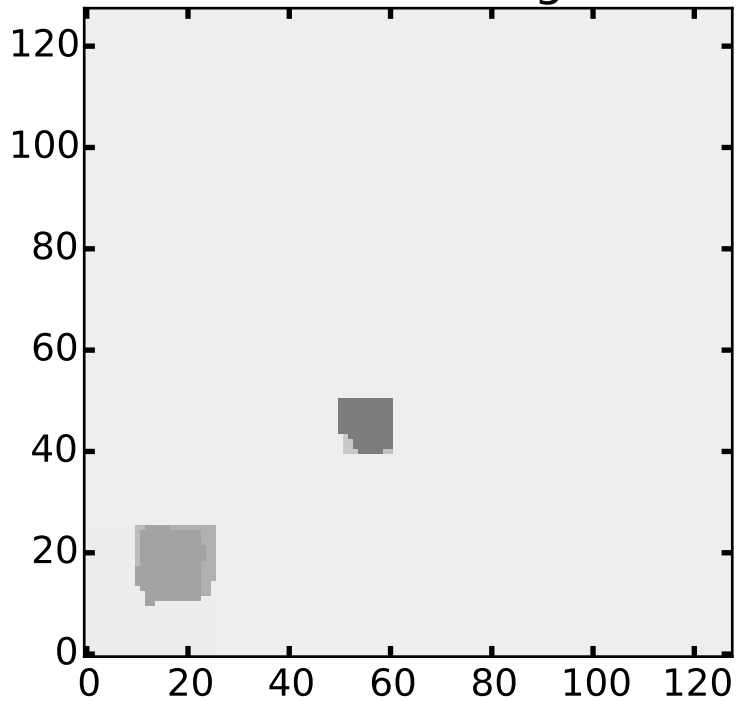
Smoothed Weights
