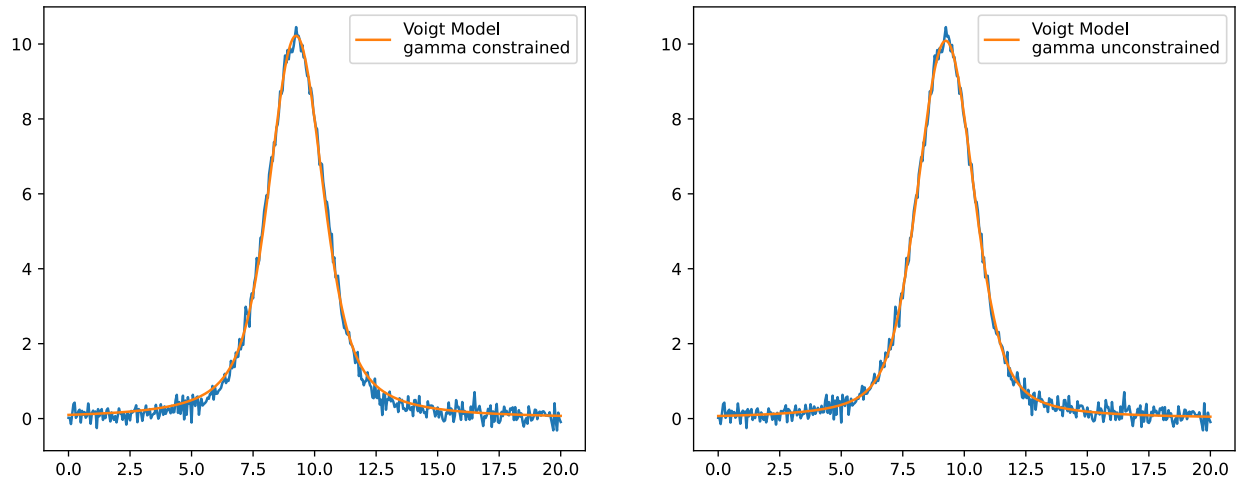
Fit to peak with Voigt model (left) and Voigt model with gamma varying independently of sigma (right).
