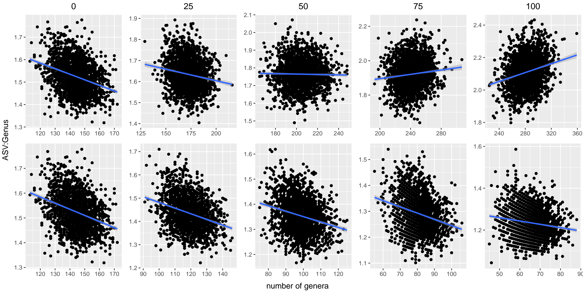
Poisson dataset, lambda = 0.01
